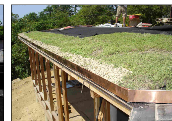
3/4 clean stone as ballast edge *Option pending detail
