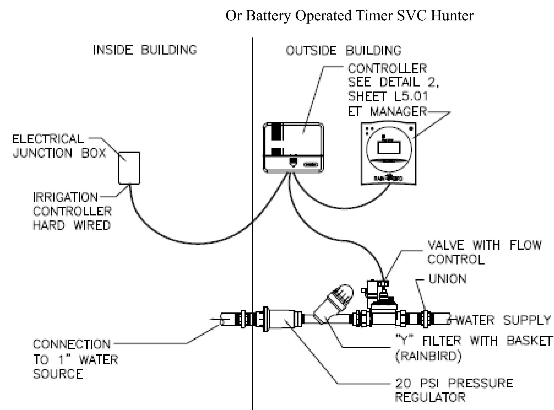
1 CONTROLLER AND ET SYSTEM TO VALVE ELECTRICAL CONNECTION NTS
