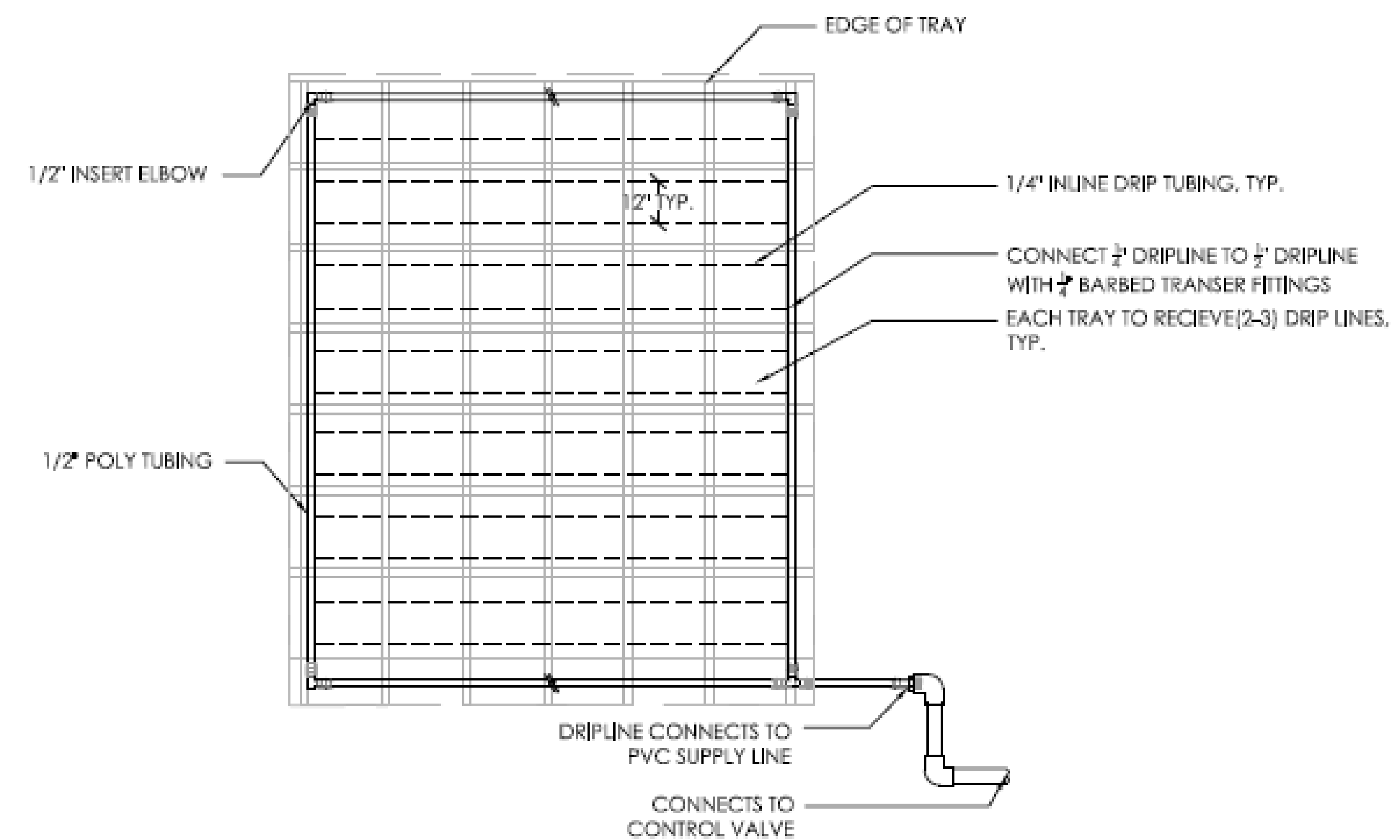
2 DRIP IRRIGATION LAYOUT NTS
